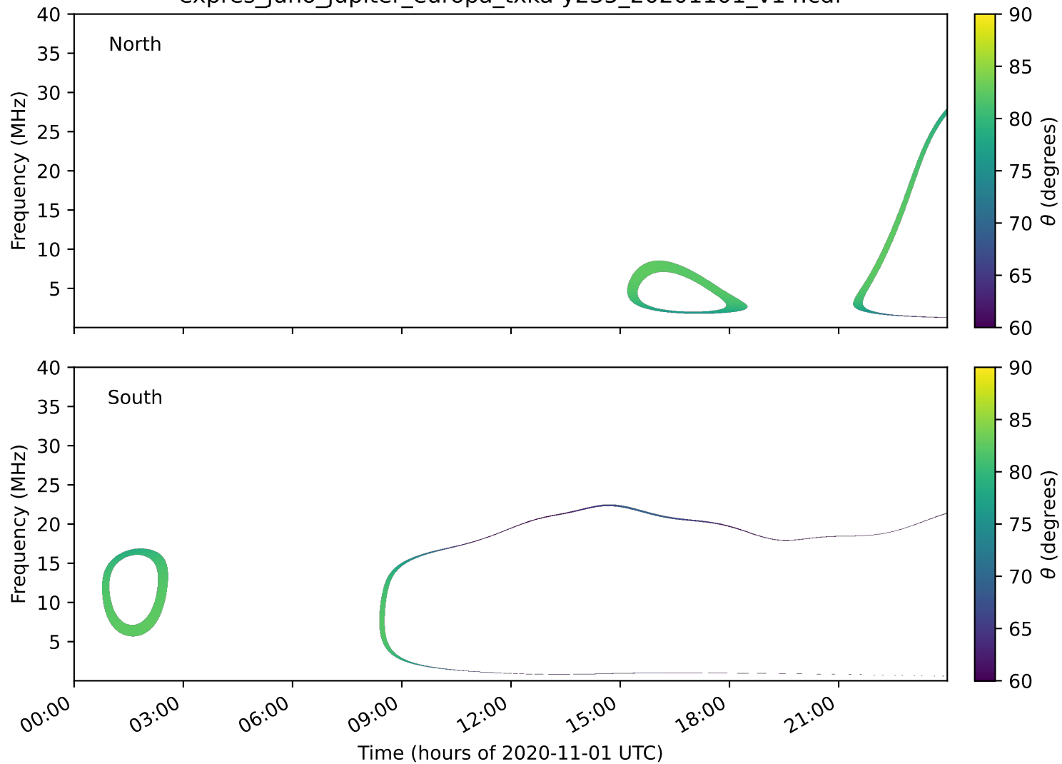
expres_juno_jupiter_europa_txka-y235_20201101_v14.cdf
