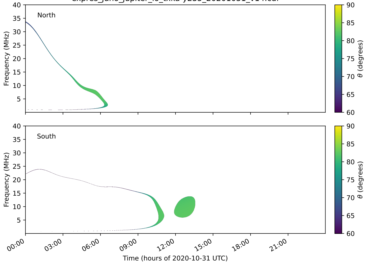
expres_juno_jupiter_io_txka-y235_20201031_v14.cdf
