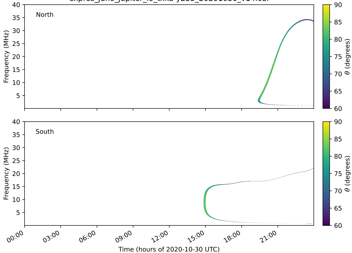
expres_juno_jupiter_io_txka-y235_20201030_v14.cdf
