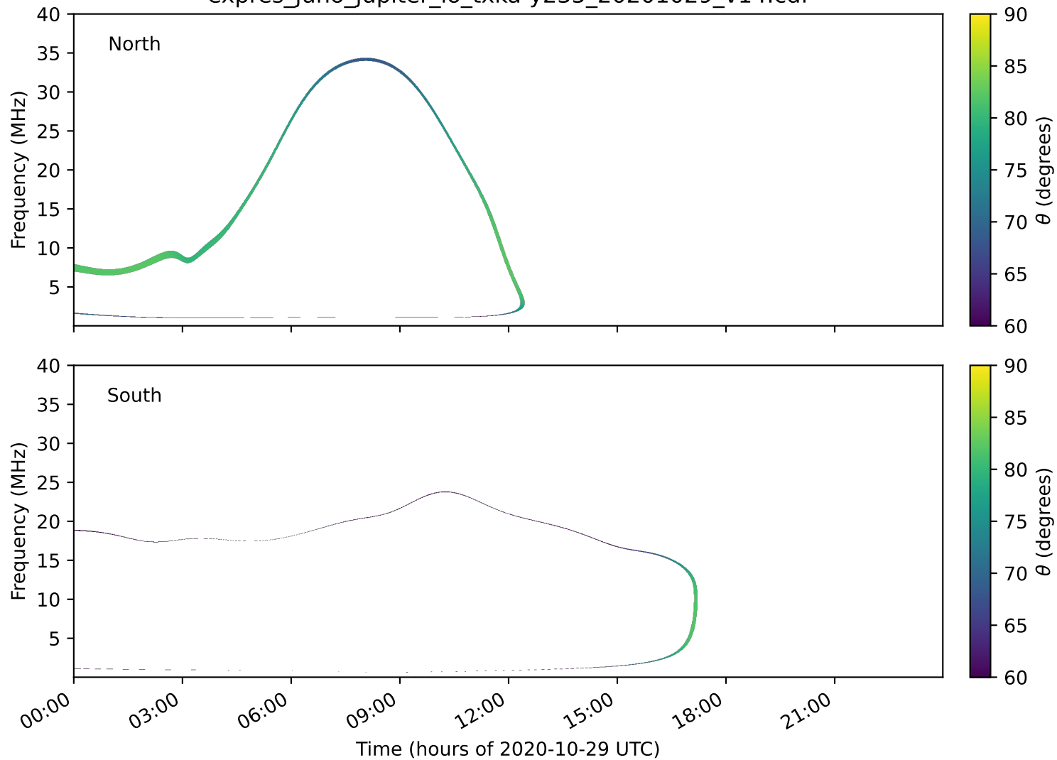
expres_juno_jupiter_io_txka-y235_20201029_v14.cdf
