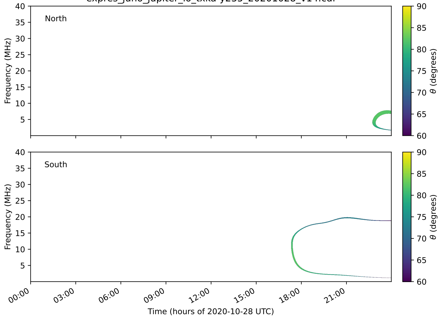
expres_juno_jupiter_io_txka-y235_20201028_v14.cdf
