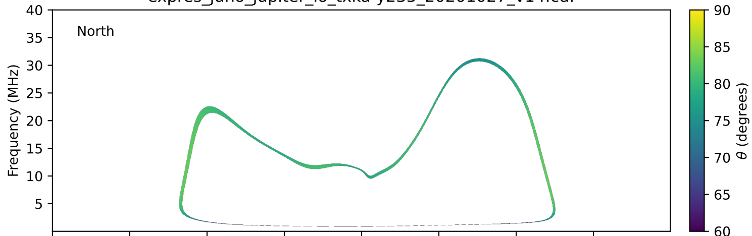
expres_juno_jupiter_io_txka-y235_20201027_v14.cdf
