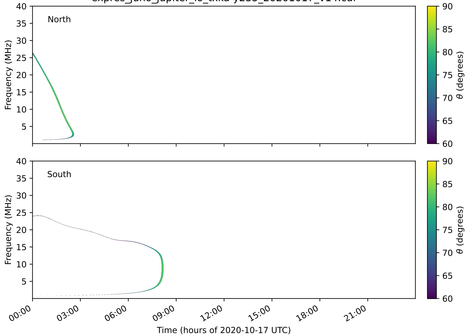
expres_juno_jupiter_io_txka-y235_20201017_v14.cdf
