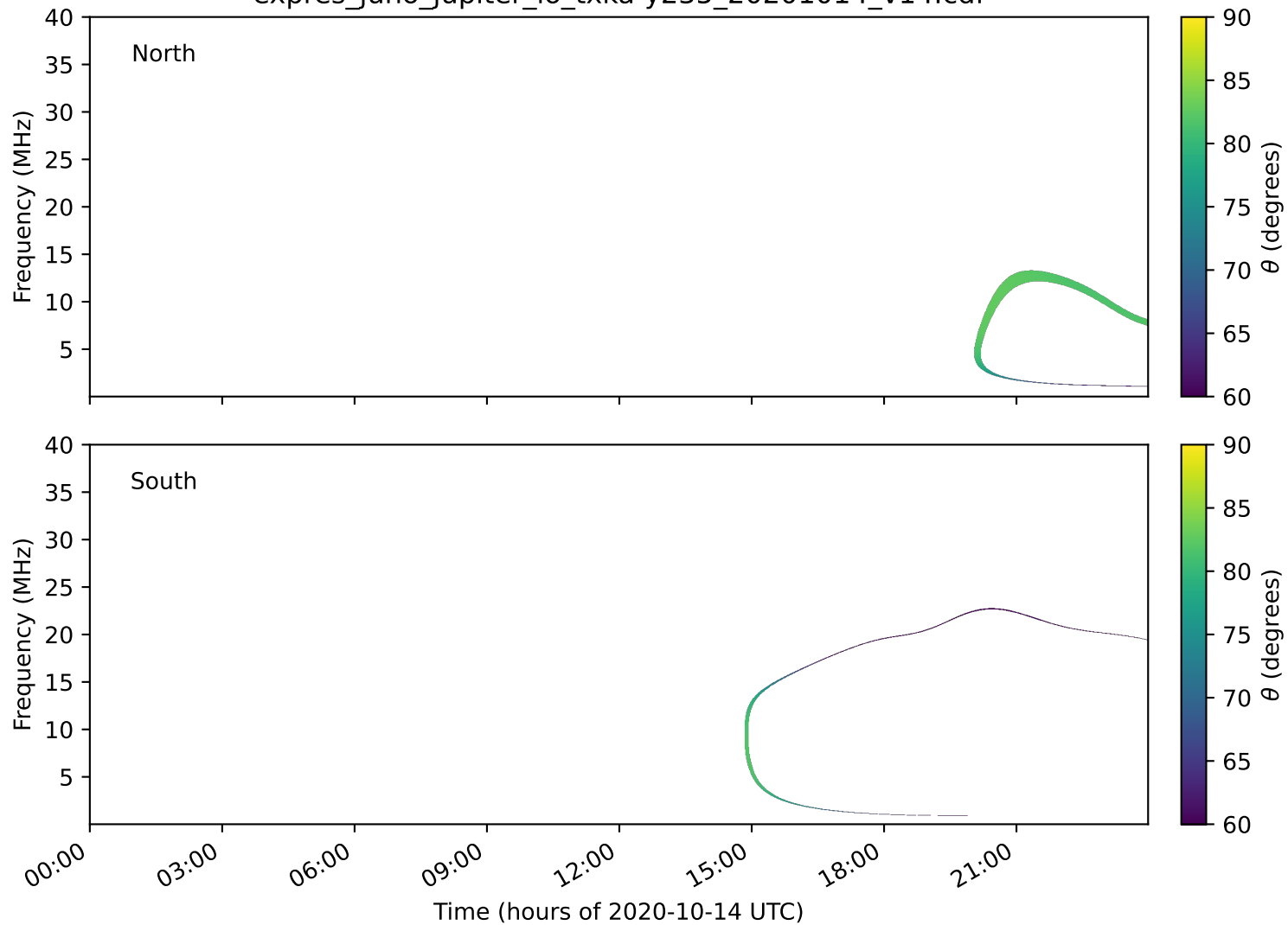
expres_juno_jupiter_io_txka-y235_20201014_v14.cdf
