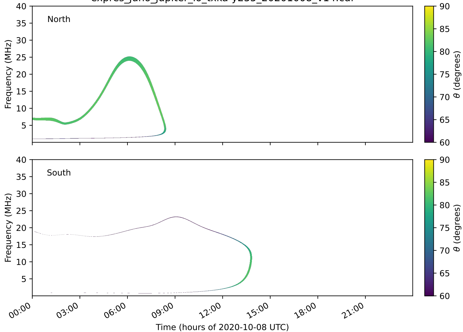
expres_juno_jupiter_io_txka-y235_20201008_v14.cdf
