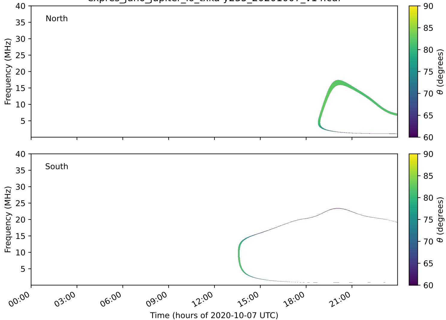
expres_juno_jupiter_io_txka-y235_20201007_v14.cdf
