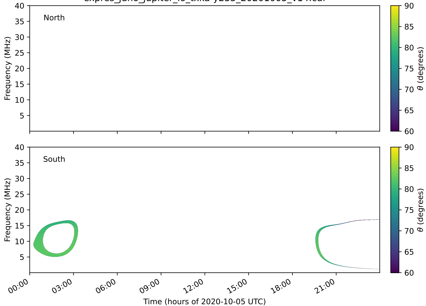
expres_juno_jupiter_io_txka-y235_20201005_v14.cdf
