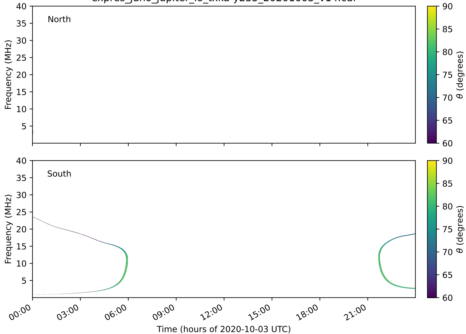
expres_juno_jupiter_io_txka-y235_20201003_v14.cdf
