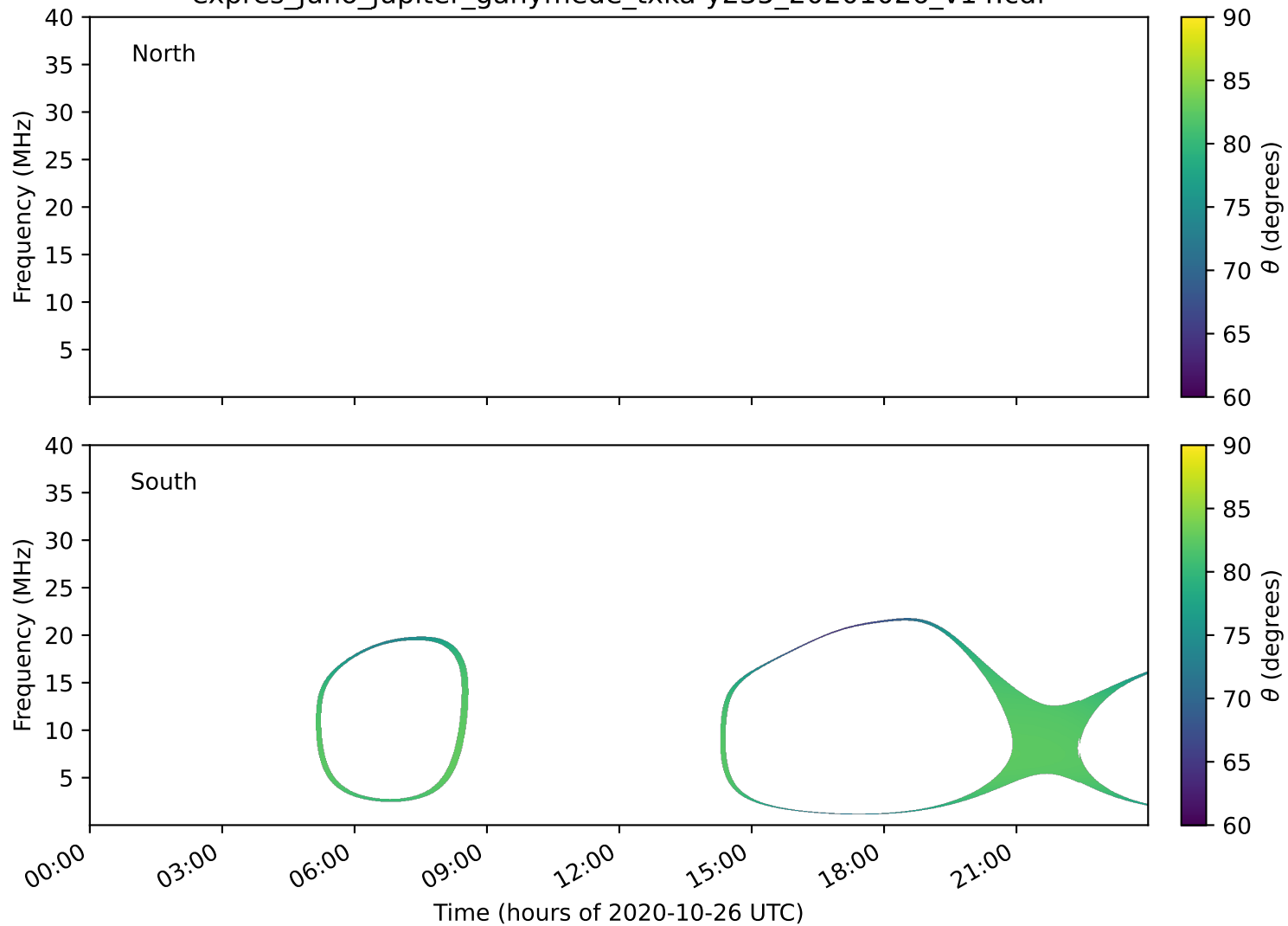
expres_juno_jupiter_ganymede_txka-y235_20201026_v14.cdf
