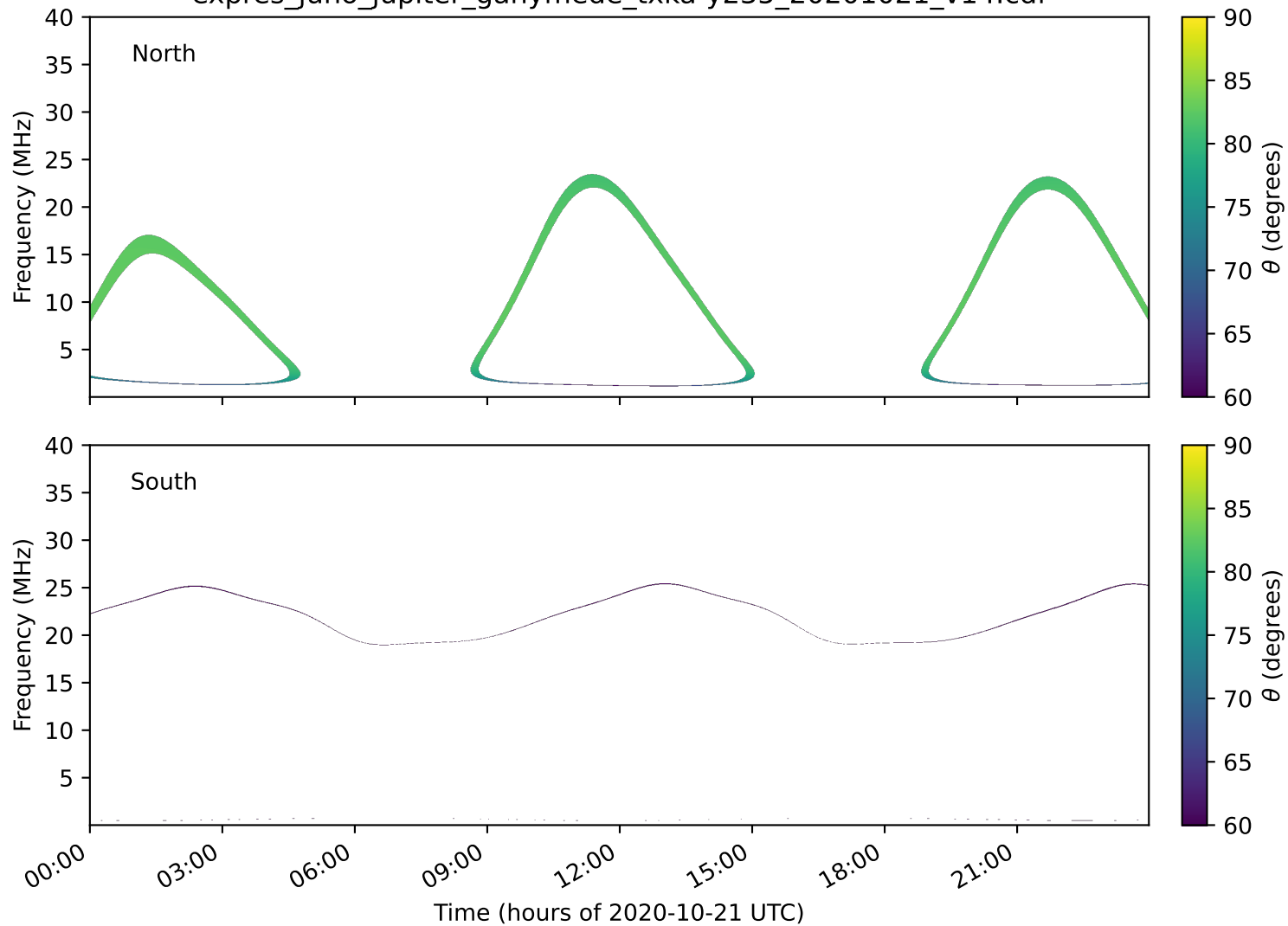
expres_juno_jupiter_ganymede_txka-y235_20201021_v14.cdf
