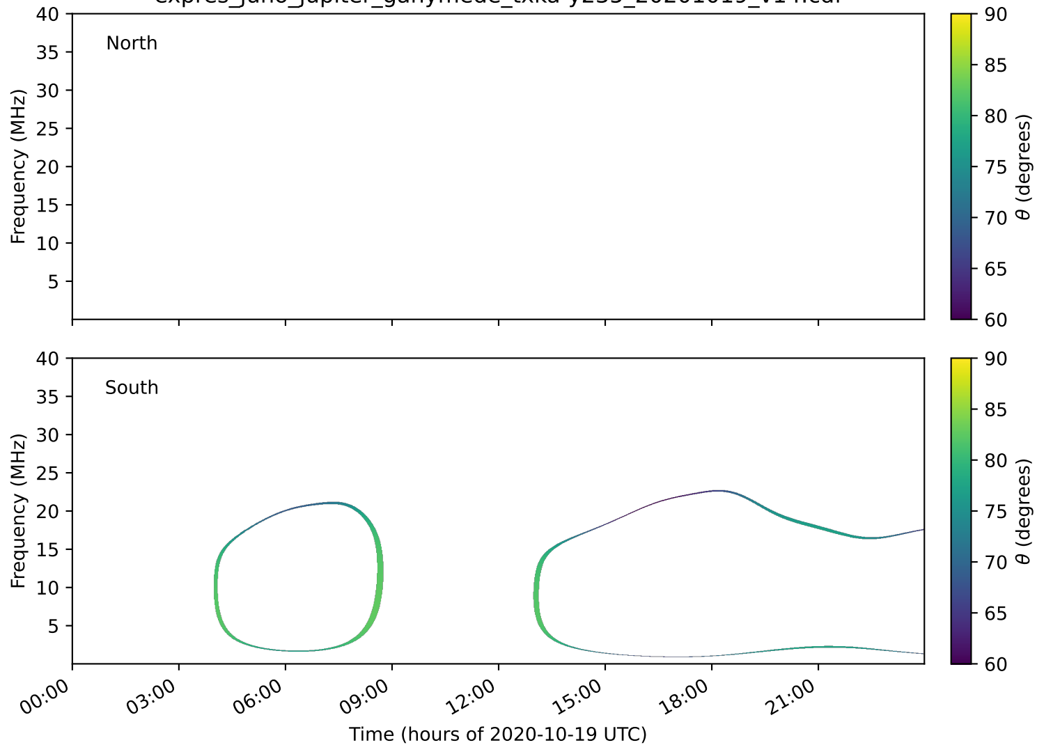
expres_juno_jupiter_ganymede_txka-y235_20201019_v14.cdf
