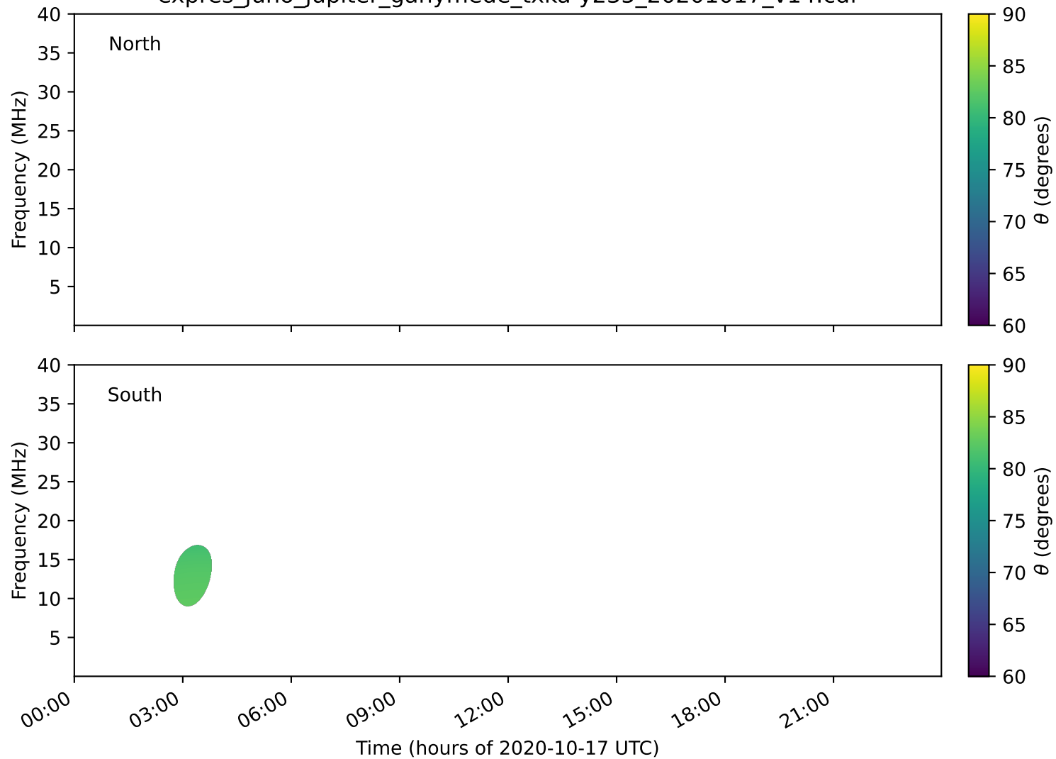
expres_juno_jupiter_ganymede_txka-y235_20201017_v14.cdf
