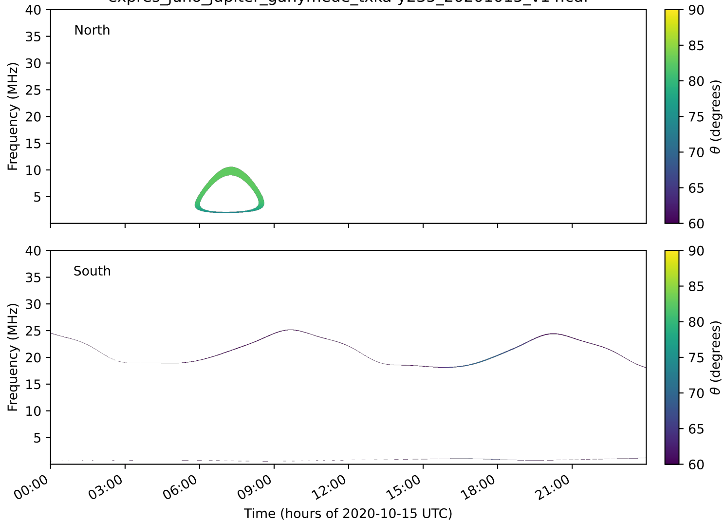
expres_juno_jupiter_ganymede_txka-y235_20201015_v14.cdf
