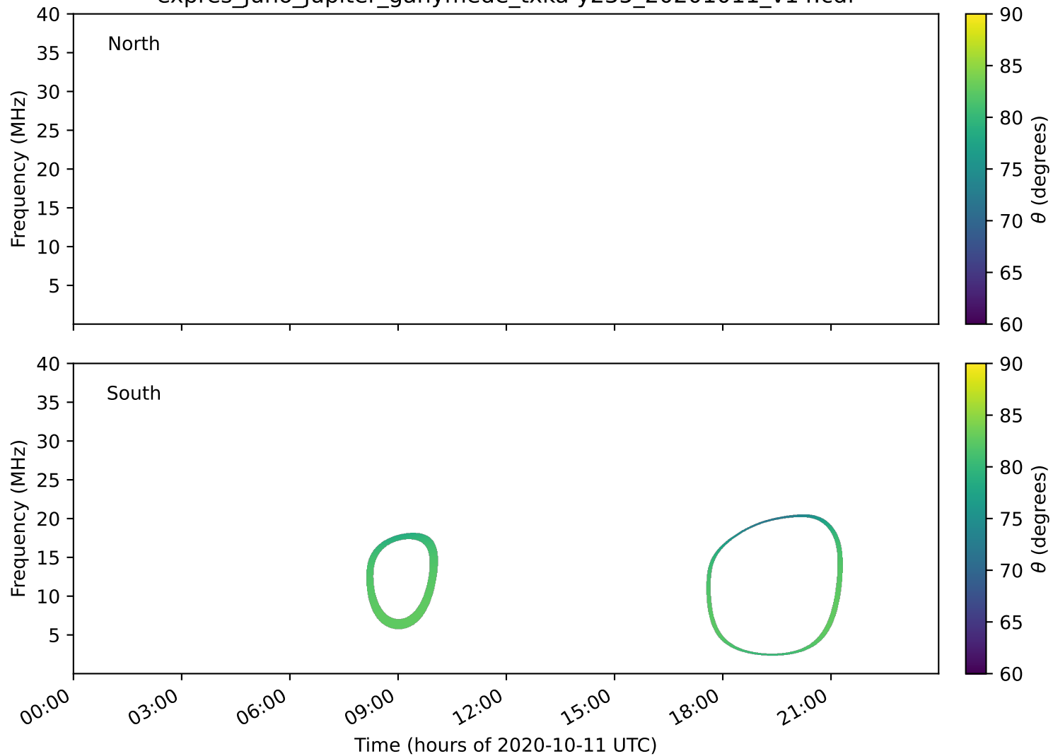
expres_juno_jupiter_ganymede_txka-y235_20201011_v14.cdf
