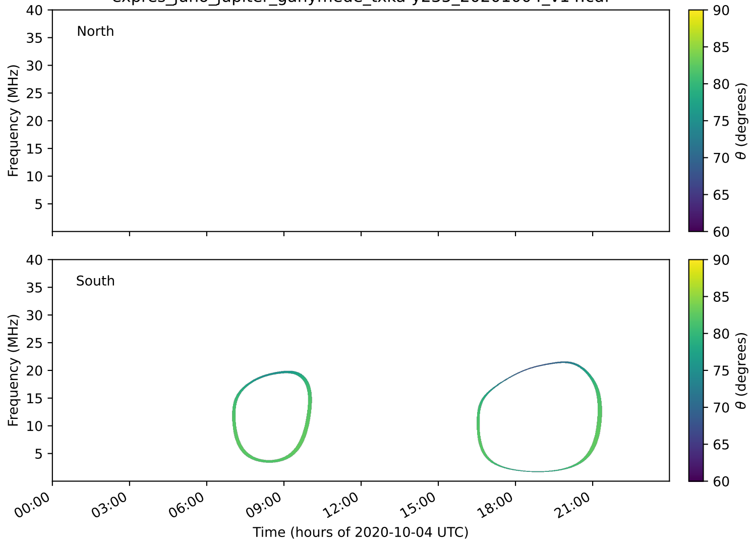
expres_juno_jupiter_ganymede_txka-y235_20201004_v14.cdf
