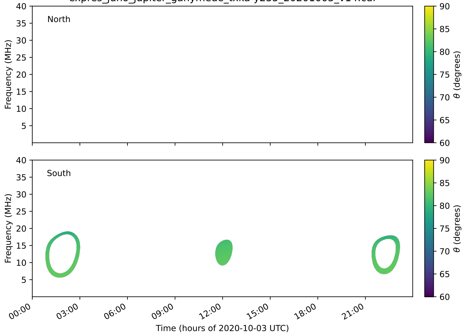
expres_juno_jupiter_ganymede_txka-y235_20201003_v14.cdf
