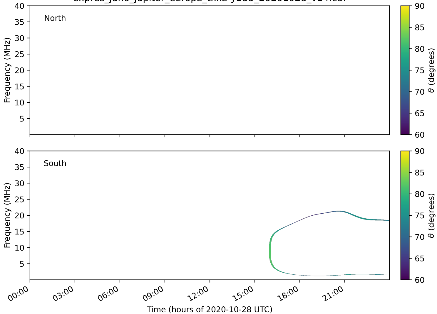
expres_juno_jupiter_europa_txka-y235_20201028_v14.cdf
