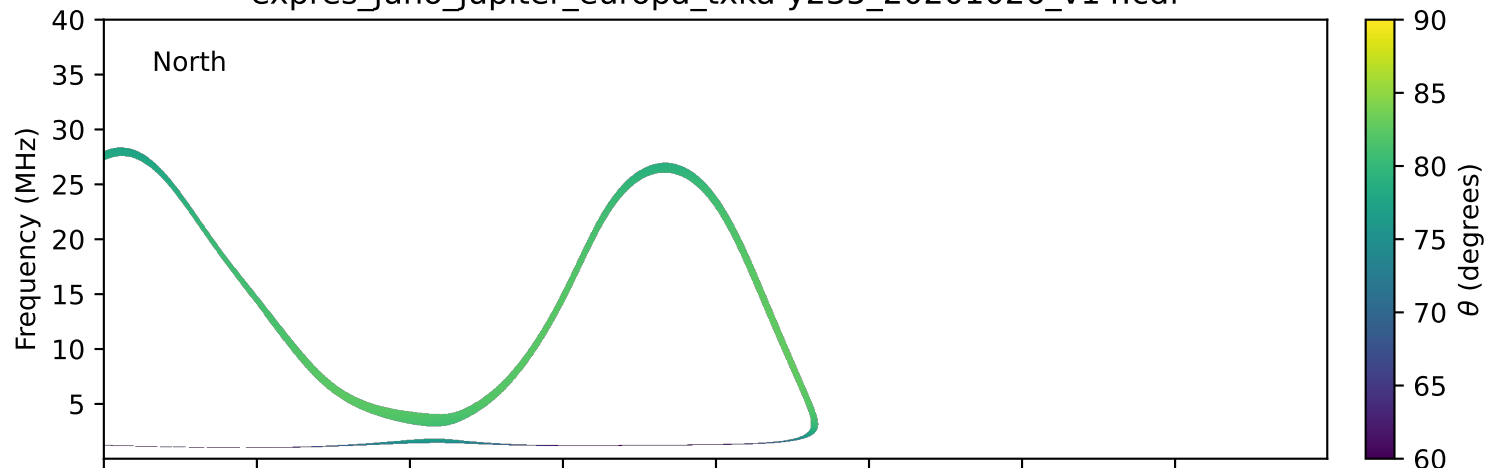
expres_juno_jupiter_europa_txka-y235_20201026_v14.cdf
