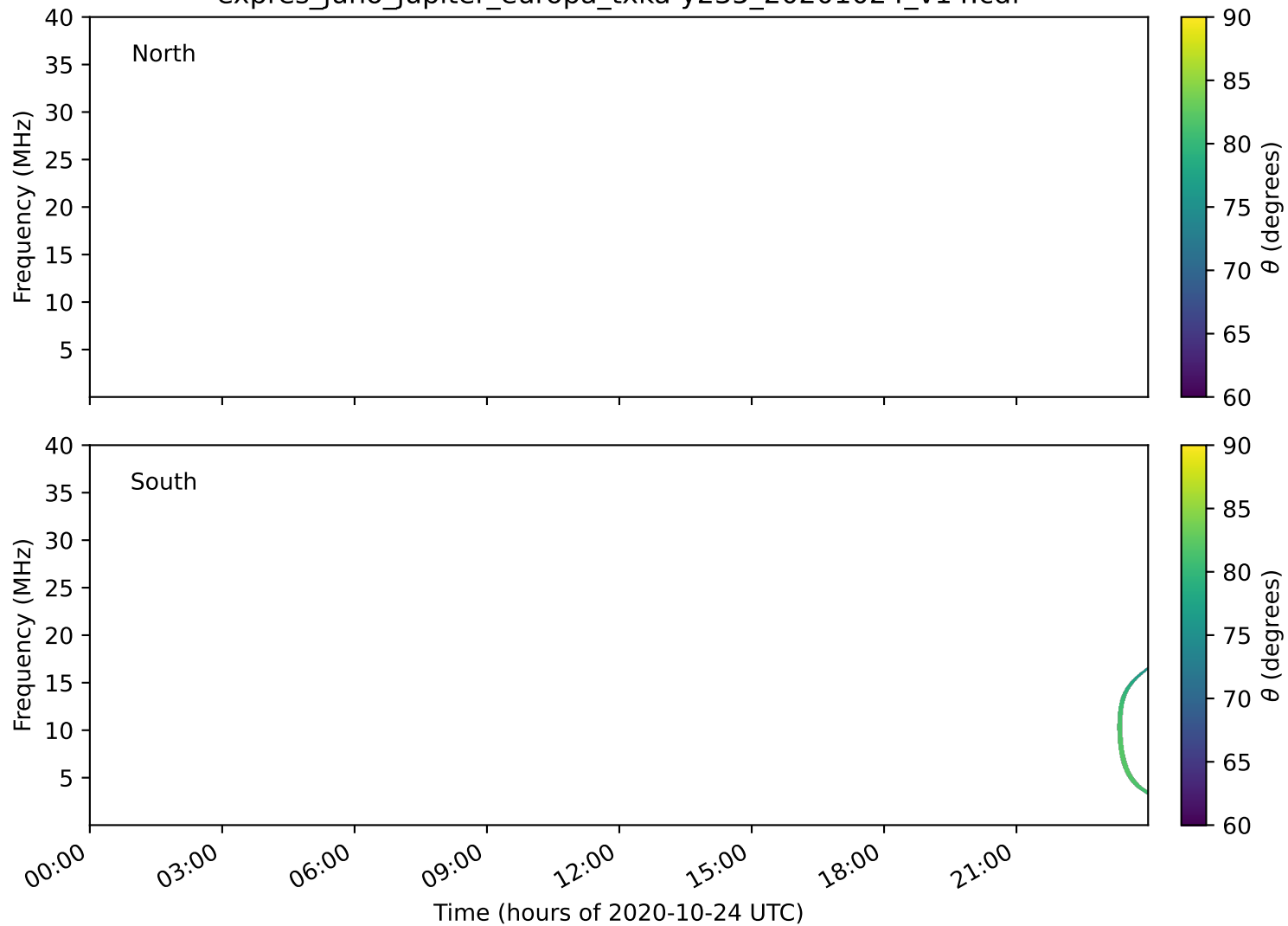
expres_juno_jupiter_europa_txka-y235_20201024_v14.cdf
