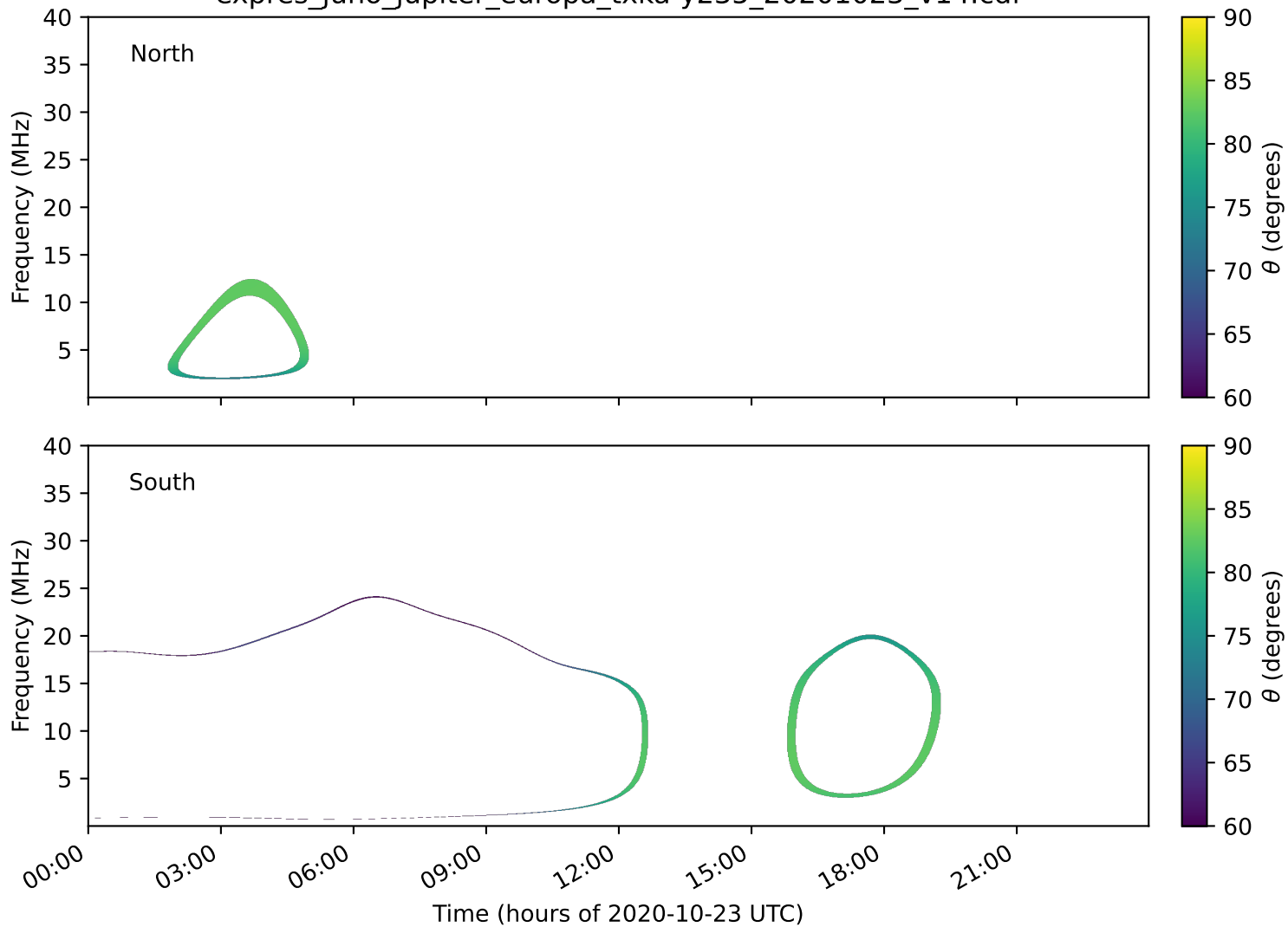
expres_juno_jupiter_europa_txka-y235_20201023_v14.cdf
