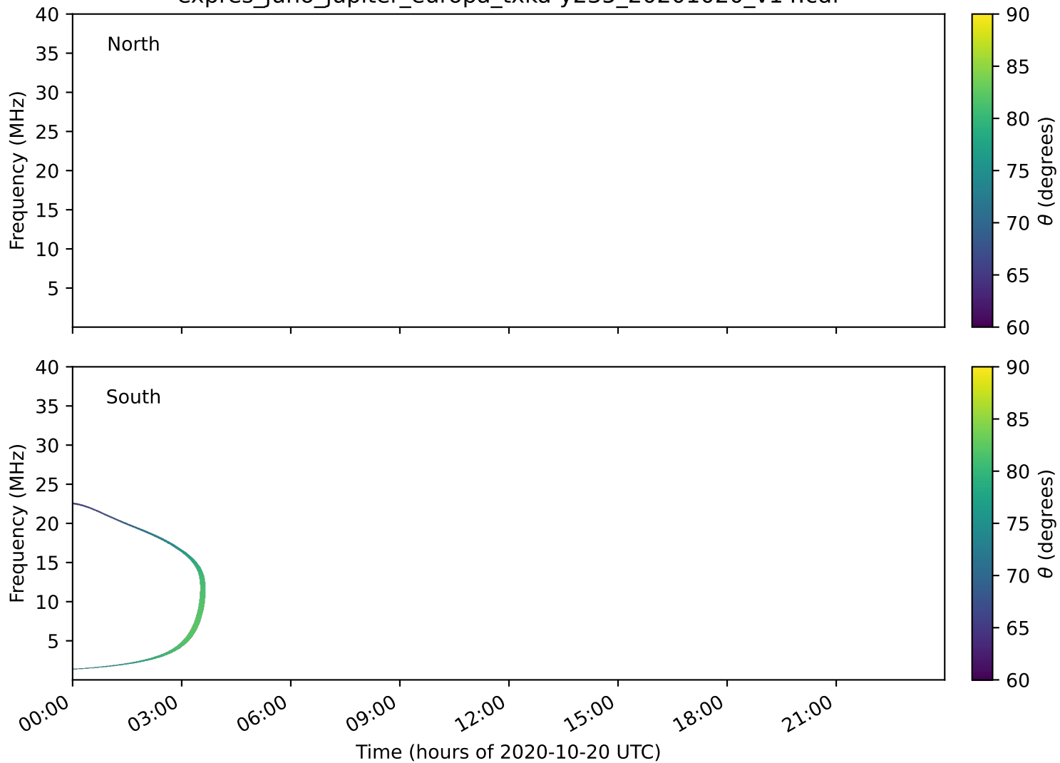
expres_juno_jupiter_europa_txka-y235_20201020_v14.cdf
