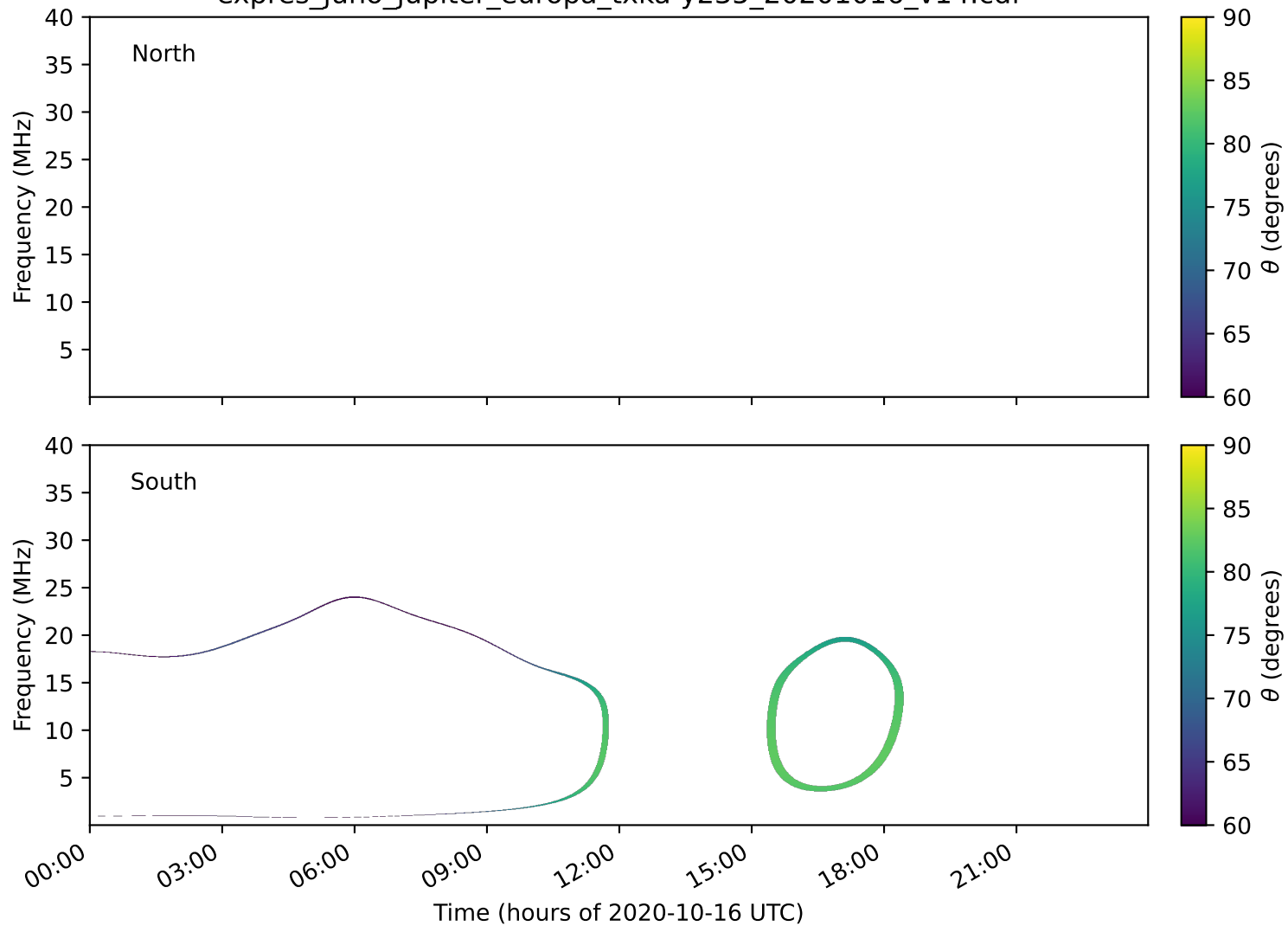
expres_juno_jupiter_europa_txka-y235_20201016_v14.cdf
