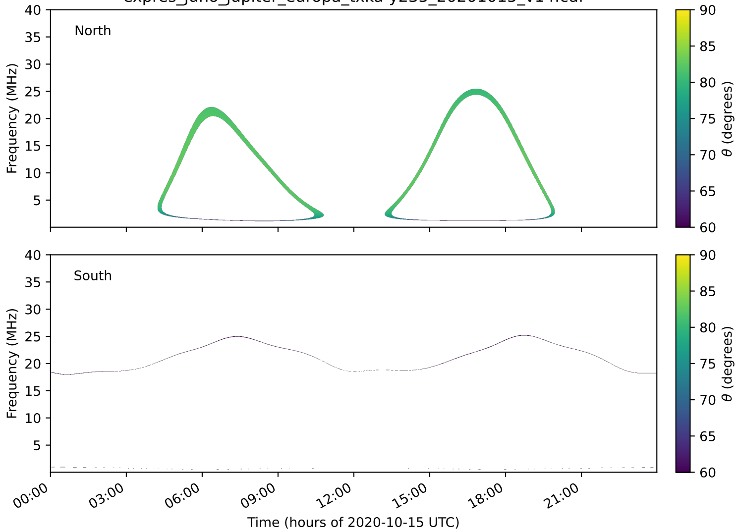
expres_juno_jupiter_europa_txka-y235_20201015_v14.cdf
