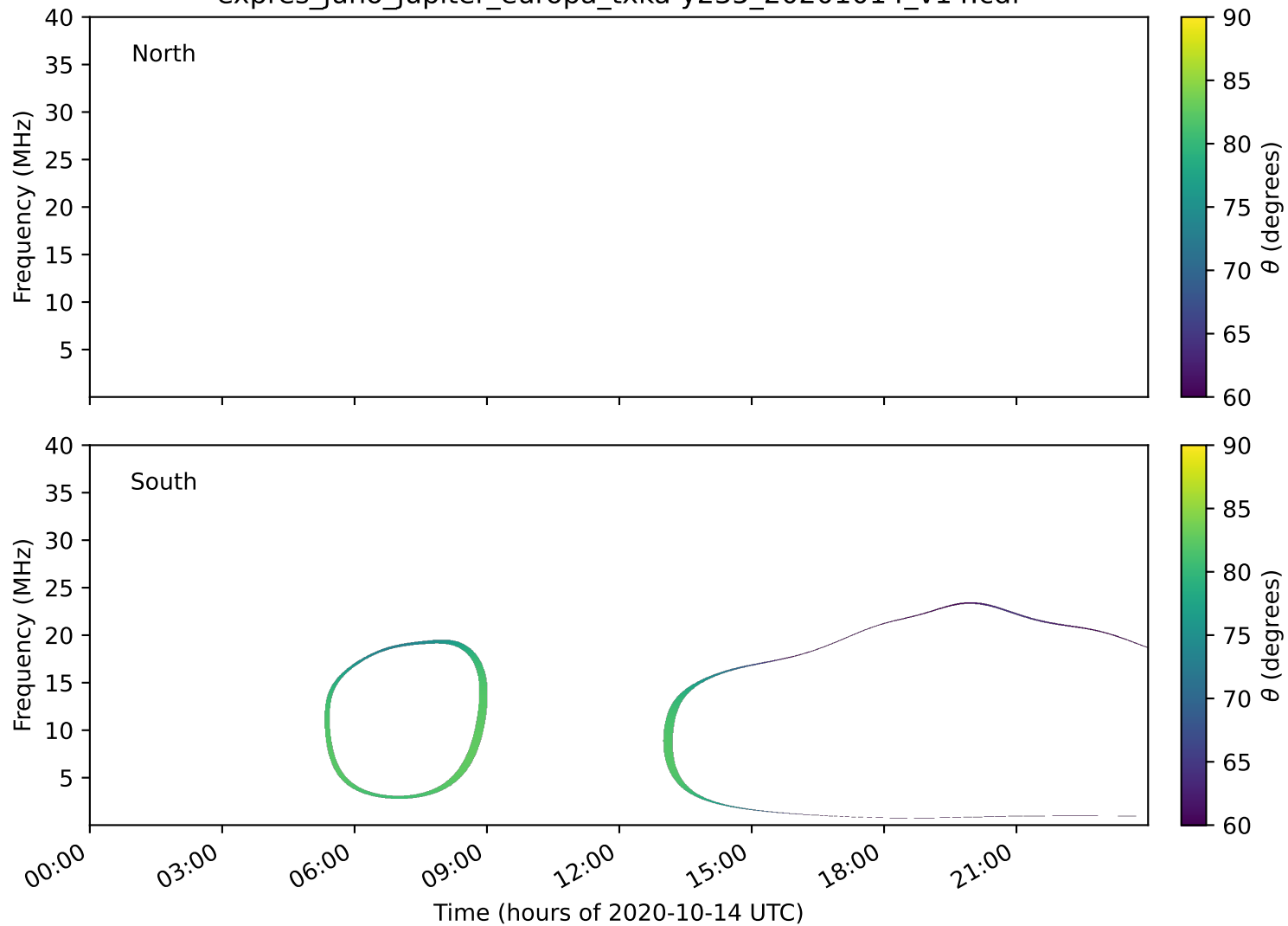
expres_juno_jupiter_europa_txka-y235_20201014_v14.cdf
