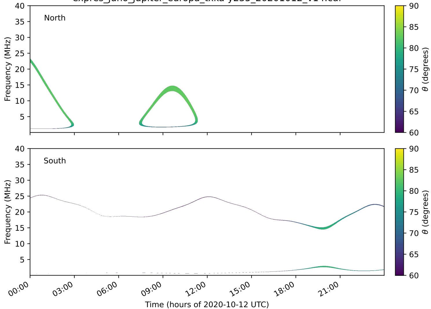
expres_juno_jupiter_europa_txka-y235_20201012_v14.cdf
