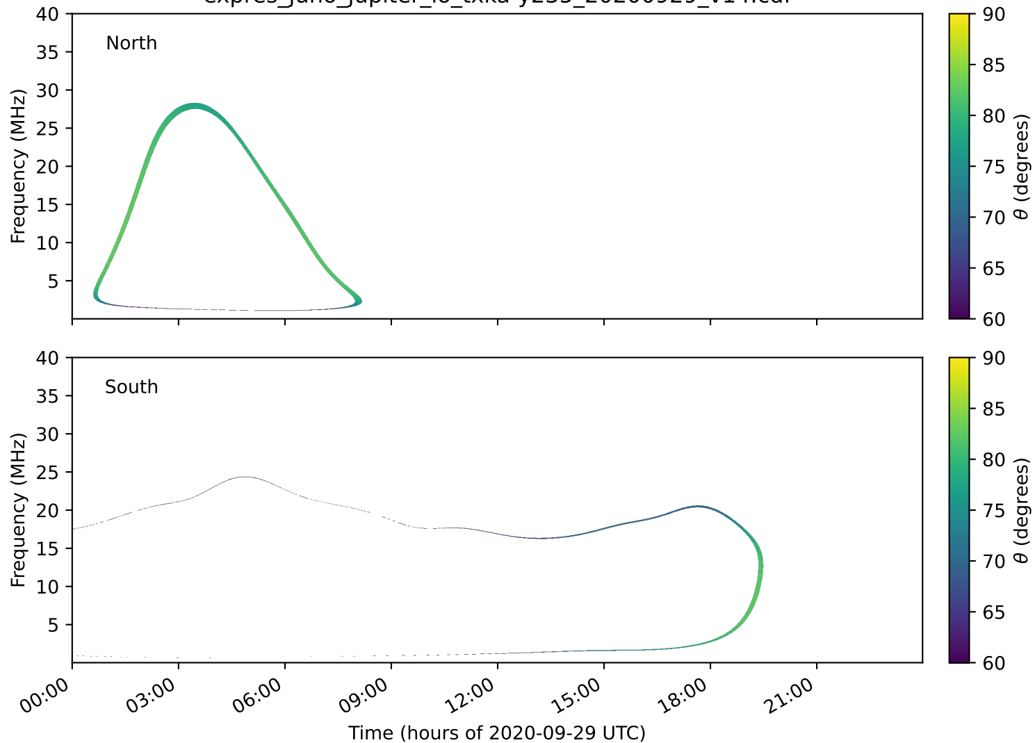
expres_juno_jupiter_io_txka-y235_20200929_v14.cdf
