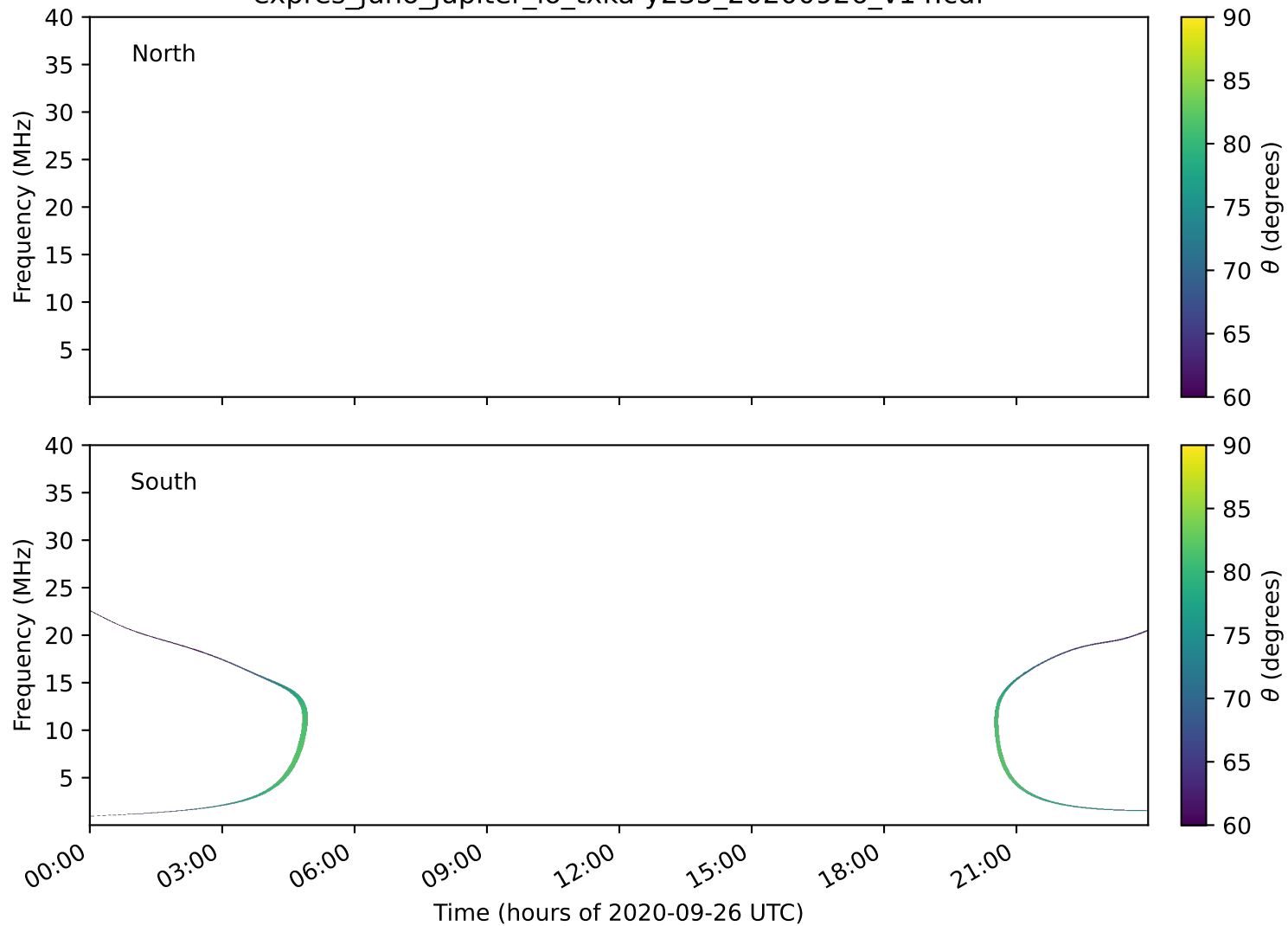
expres_juno_jupiter_io_txka-y235_20200926_v14.cdf
