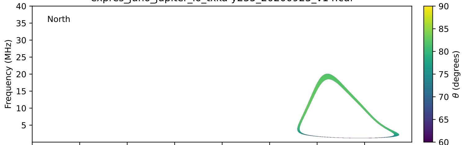
expres_juno_jupiter_io_txka-y235_20200923_v14.cdf
