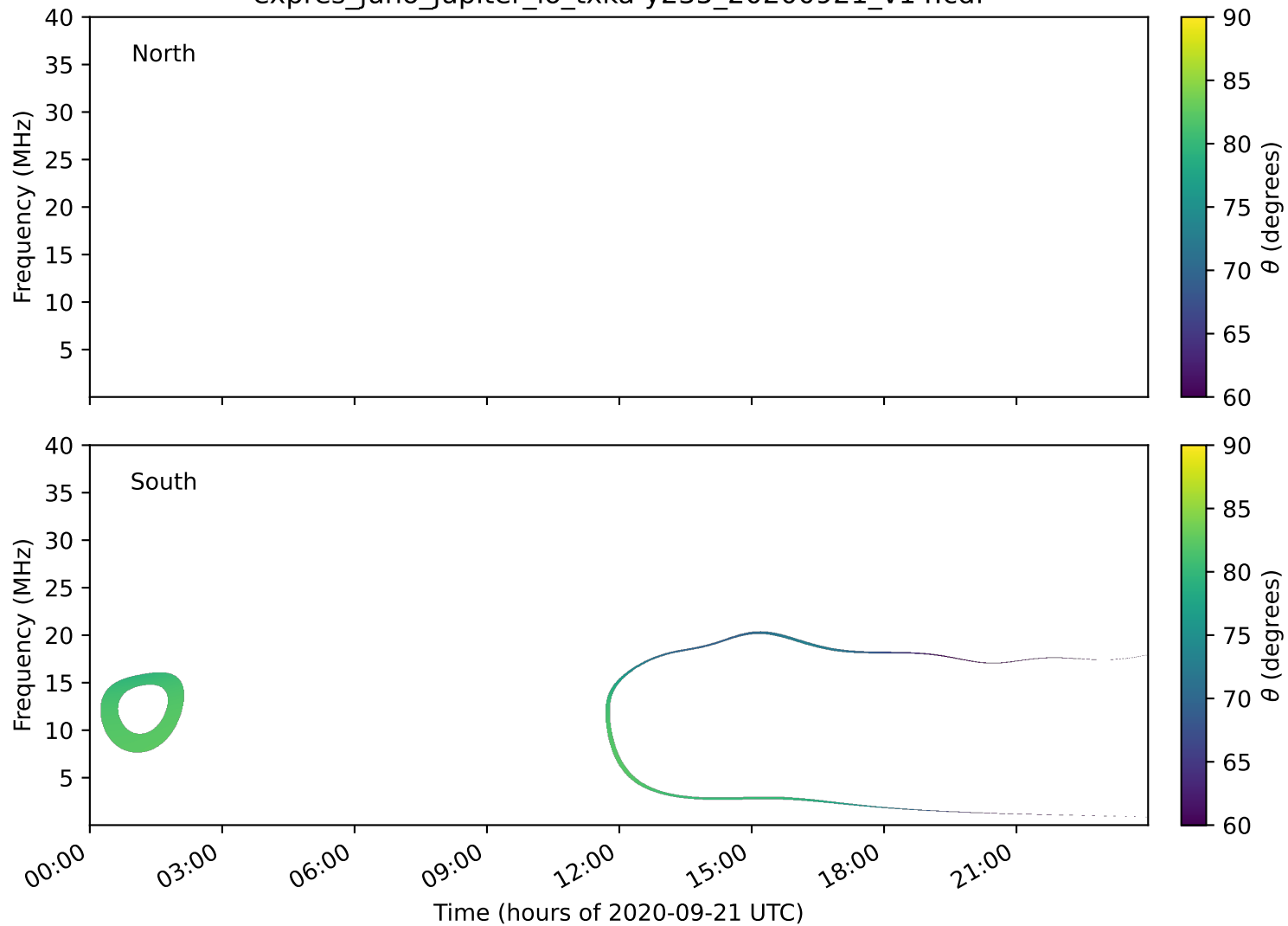
expres_juno_jupiter_io_txka-y235_20200921_v14.cdf
