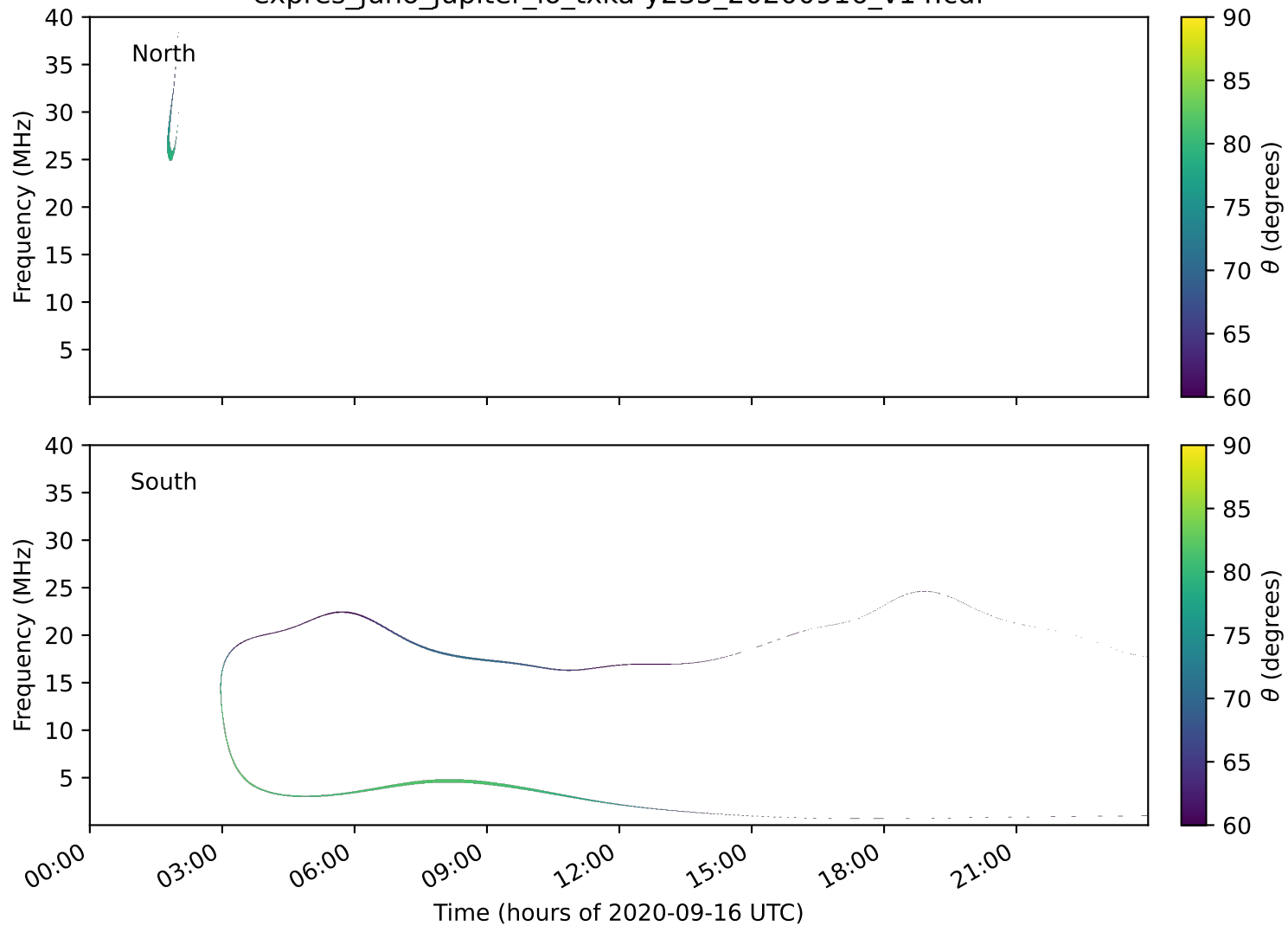
expres_juno_jupiter_io_txka-y235_20200916_v14.cdf
