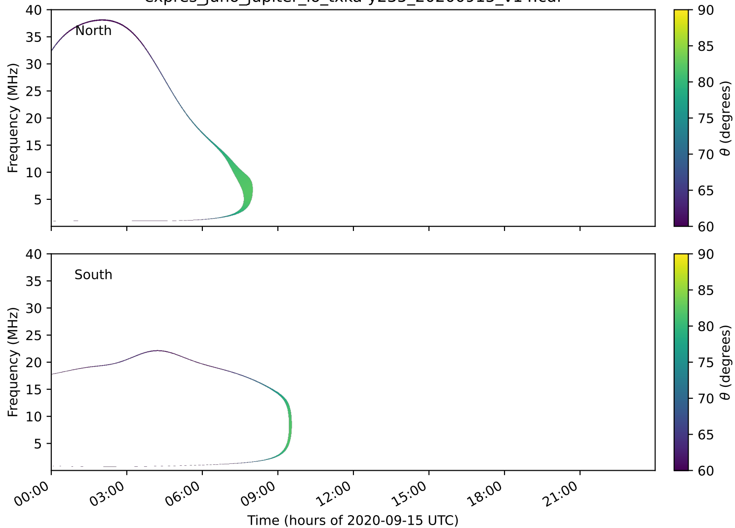
expres_juno_jupiter_io_txka-y235_20200915_v14.cdf
