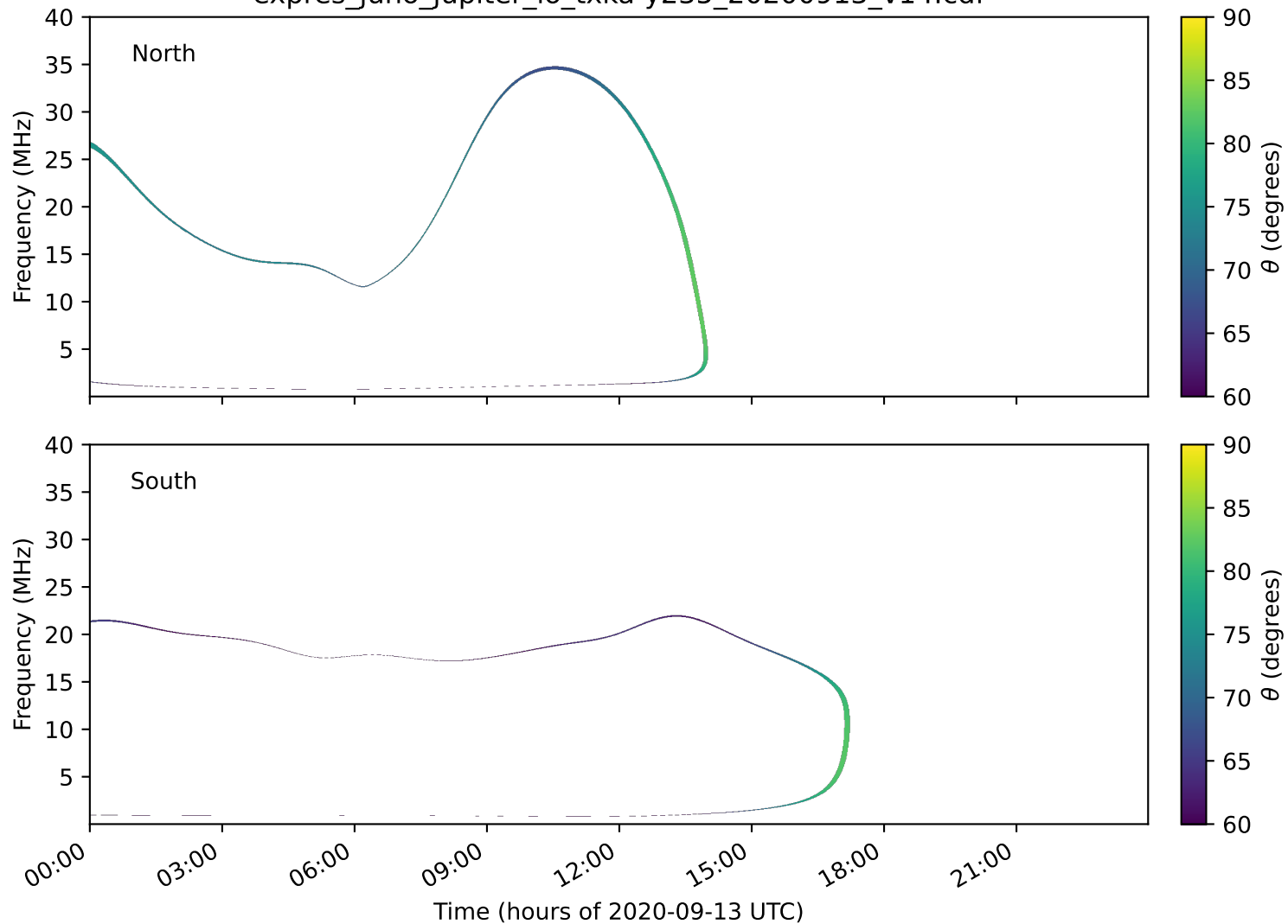
expres_juno_jupiter_io_txka-y235_20200913_v14.cdf
