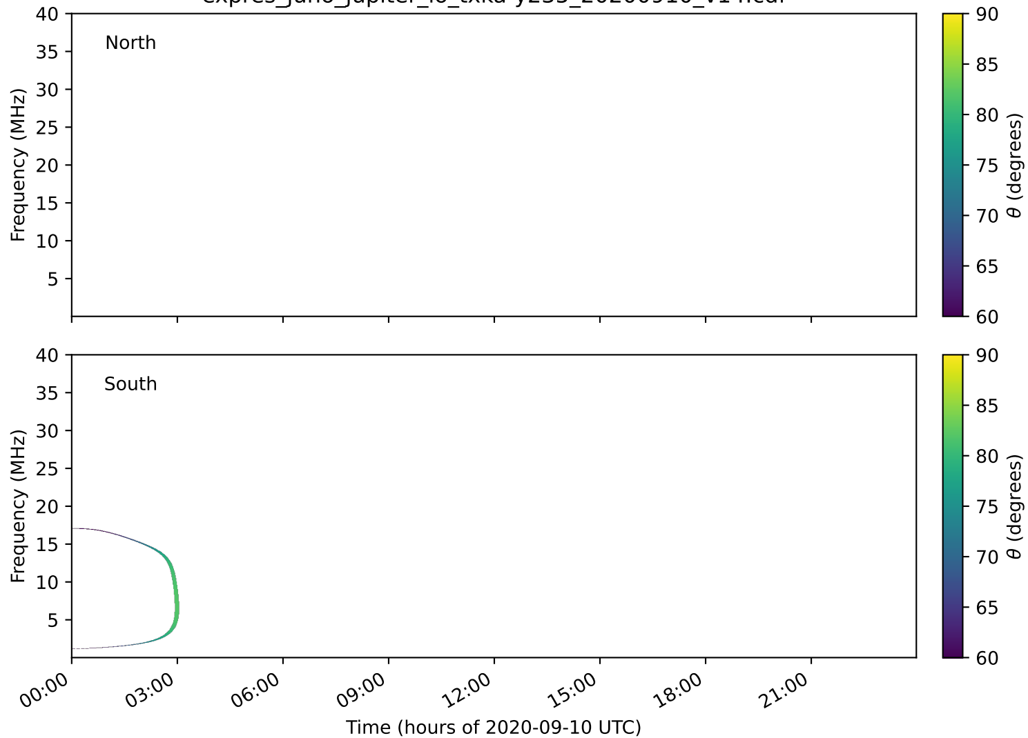
expres_juno_jupiter_io_txka-y235_20200910_v14.cdf
