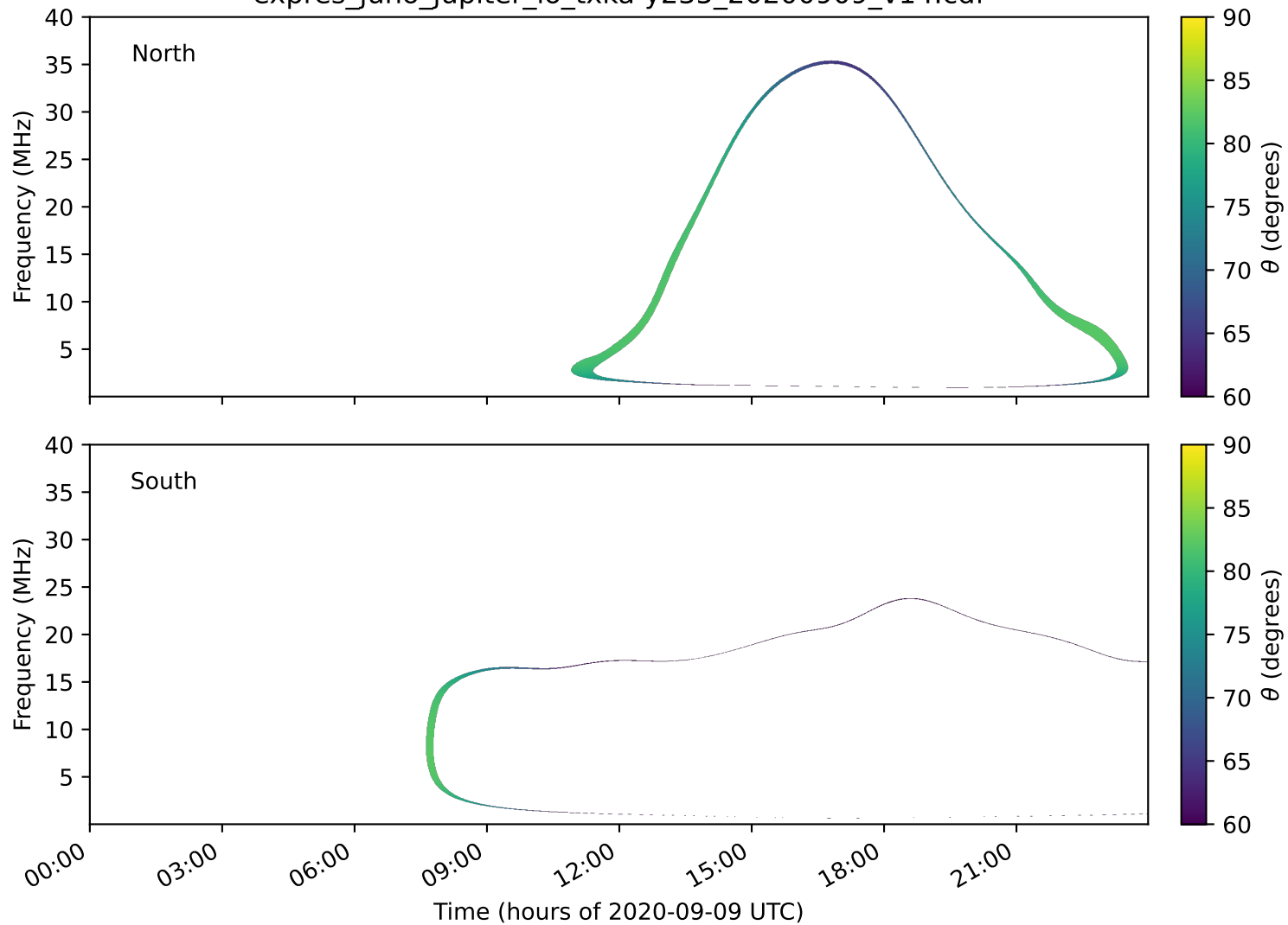
expres_juno_jupiter_io_txka-y235_20200909_v14.cdf
