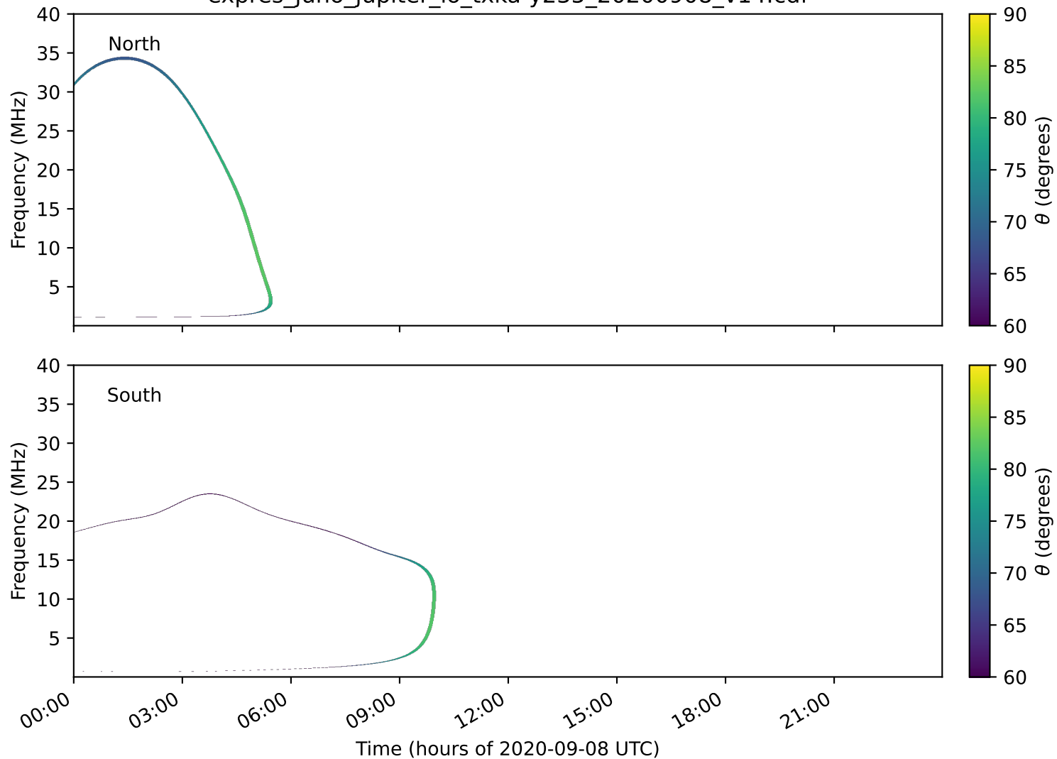
expres_juno_jupiter_io_txka-y235_20200908_v14.cdf
