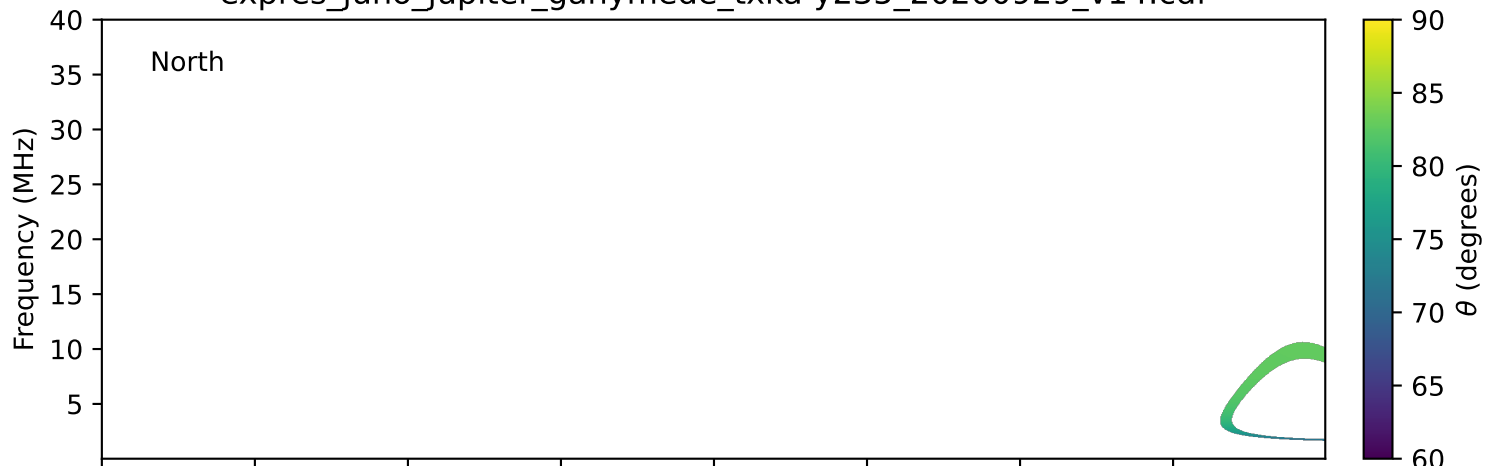
expres_juno_jupiter_ganymede_txka-y235_20200929_v14.cdf
