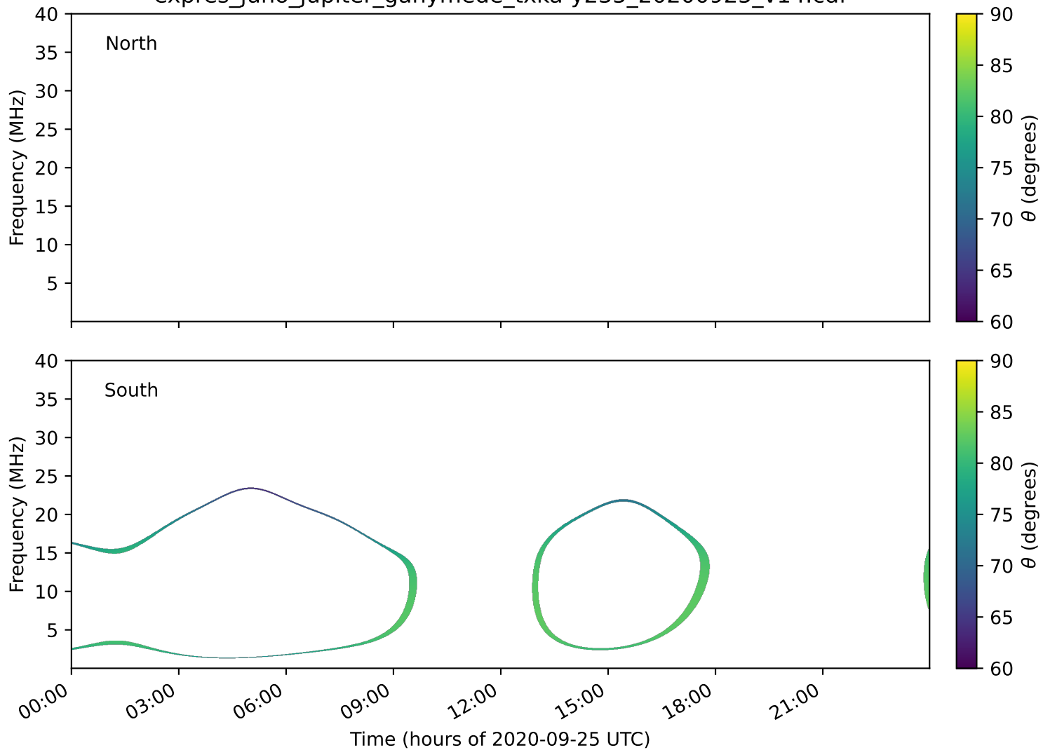
expres_juno_jupiter_ganymede_txka-y235_20200925_v14.cdf
