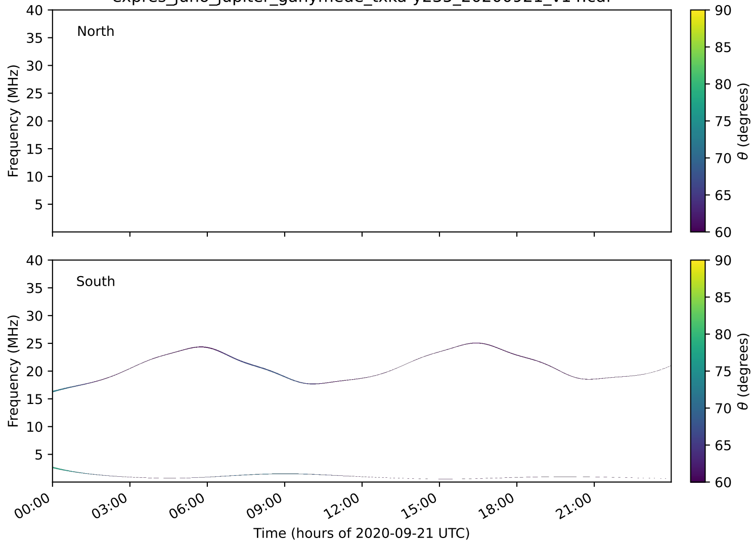
expres_juno_jupiter_ganymede_txka-y235_20200921_v14.cdf
