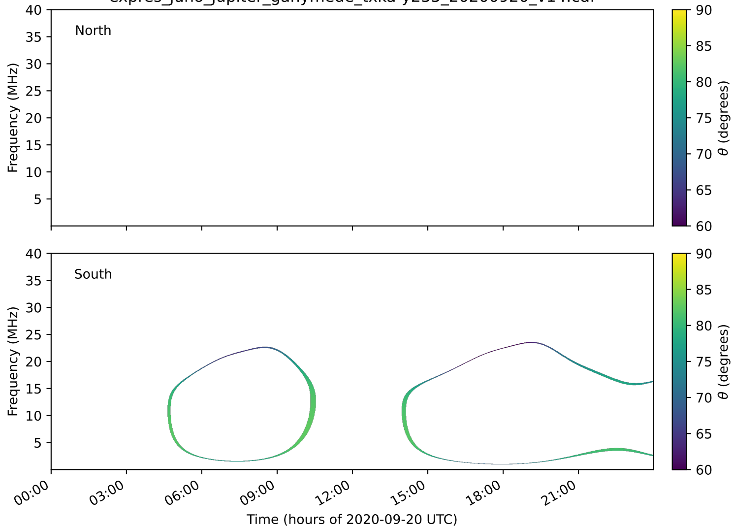
expres_juno_jupiter_ganymede_txka-y235_20200920_v14.cdf
