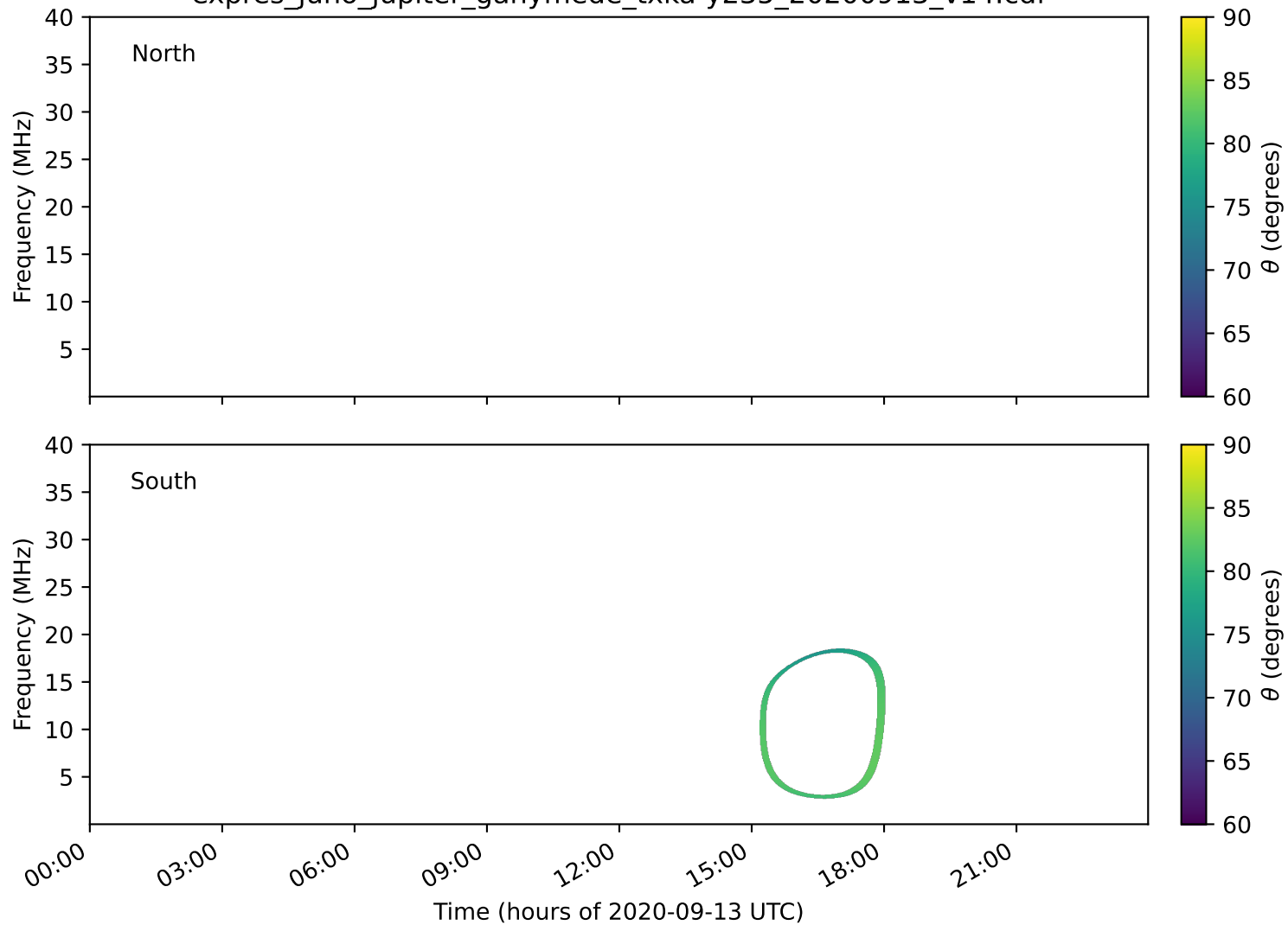
expres_juno_jupiter_ganymede_txka-y235_20200913_v14.cdf
