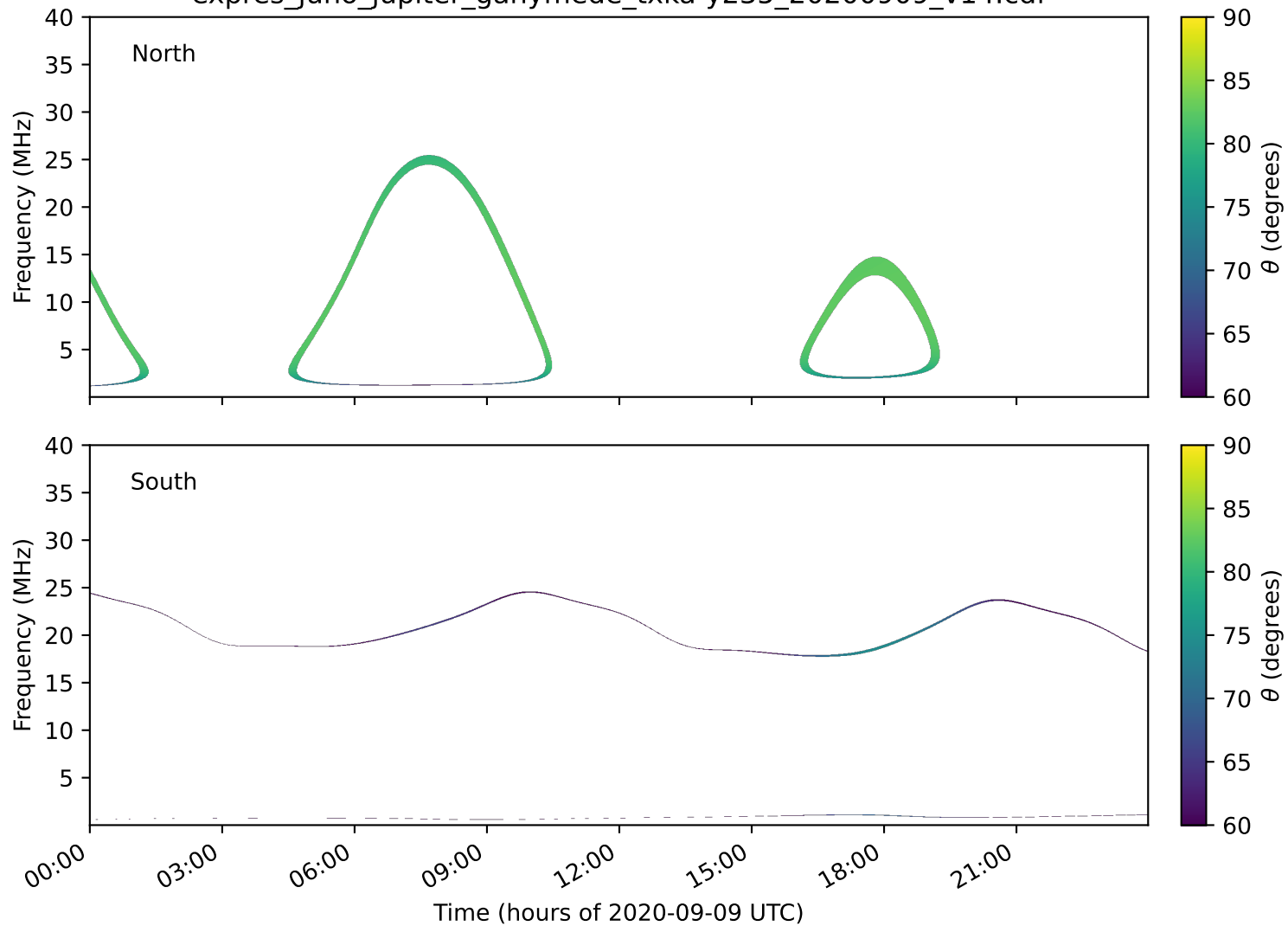
expres_juno_jupiter_ganymede_txka-y235_20200909_v14.cdf
