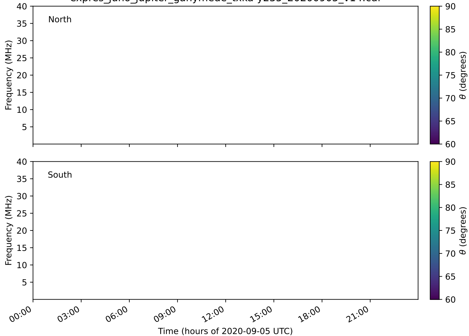
expres_juno_jupiter_ganymede_txka-y235_20200905_v14.cdf
