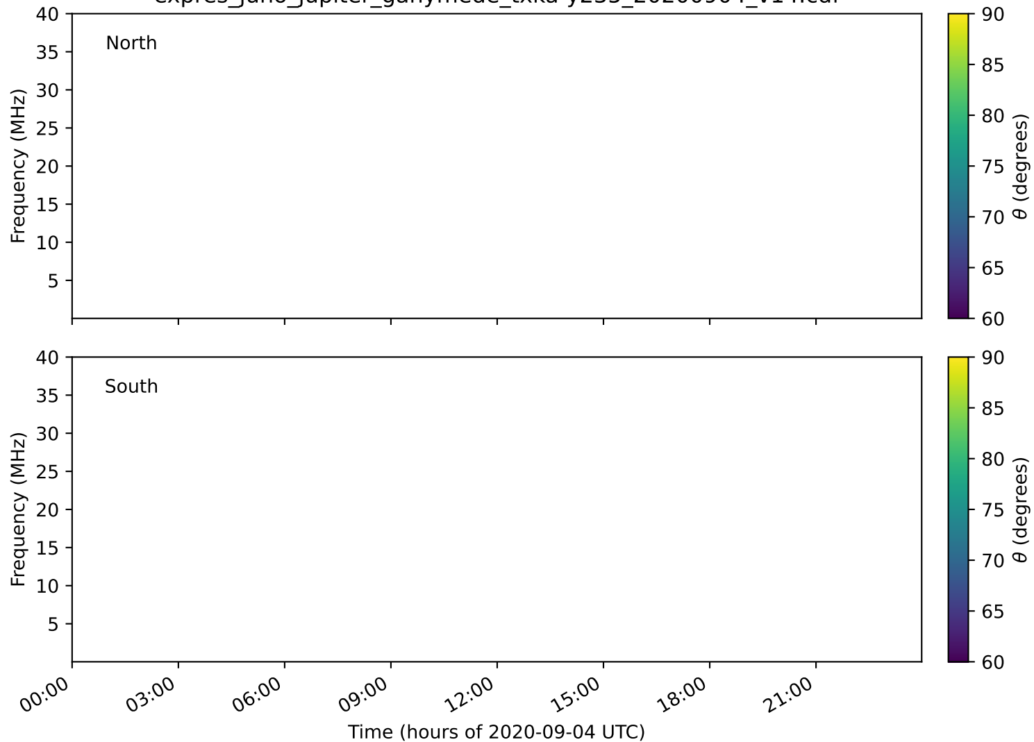
expres_juno_jupiter_ganymede_txka-y235_20200904_v14.cdf
