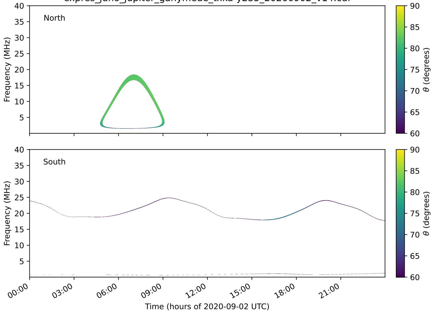
expres_juno_jupiter_ganymede_txka-y235_20200902_v14.cdf
