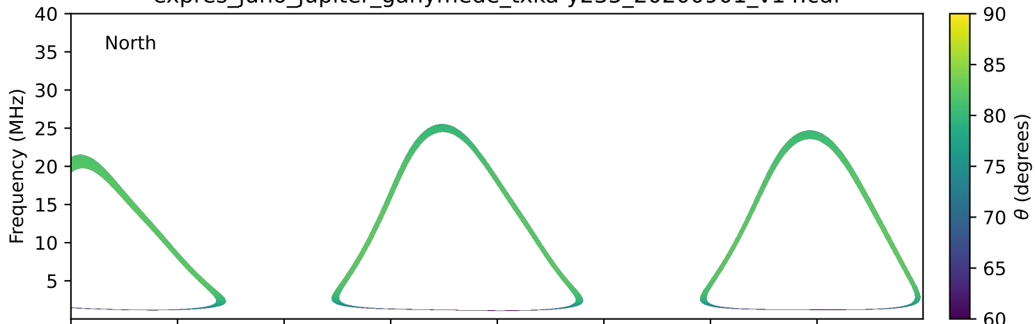
expres_juno_jupiter_ganymede_txka-y235_20200901_v14.cdf
