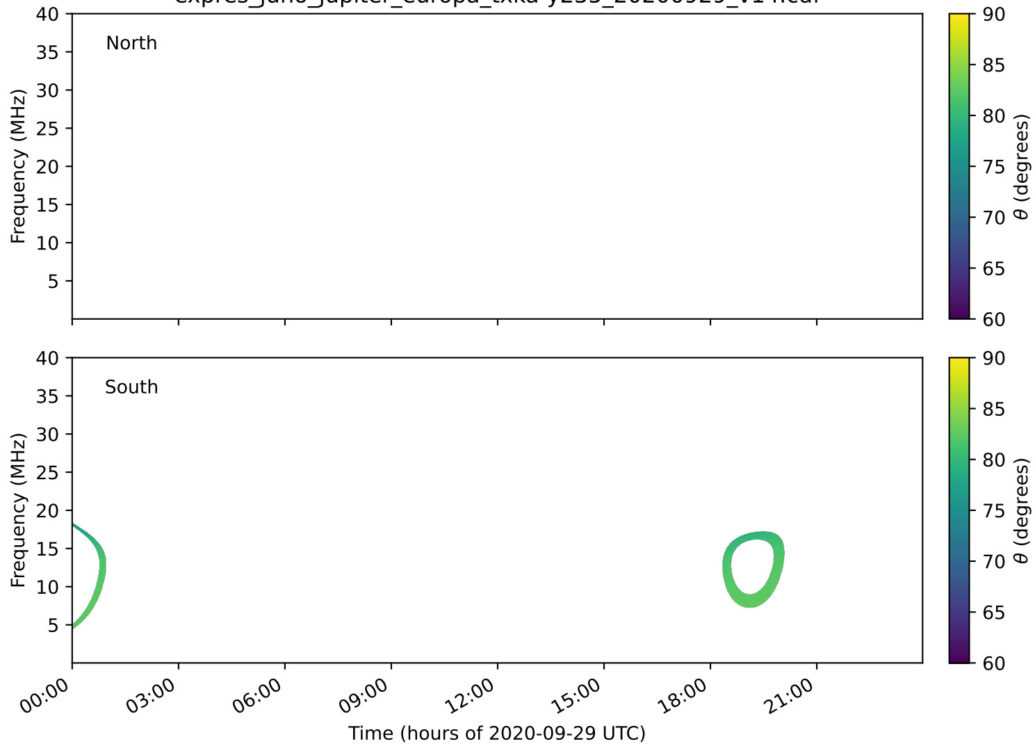
expres_juno_jupiter_europa_txka-y235_20200929_v14.cdf
